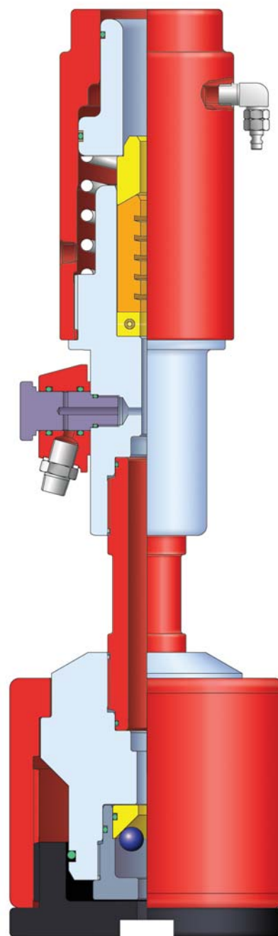
Swabbing Head
