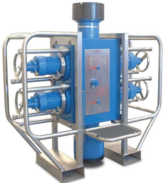
Dual Apollo Wireline Valve with Protection Frame
